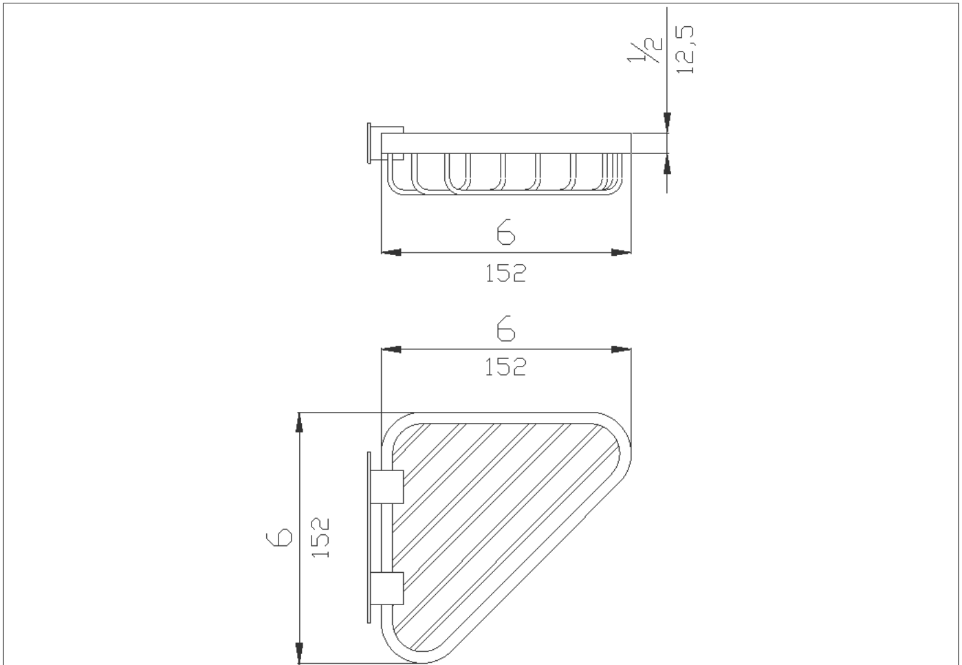
Triangular sponge-soap basket
